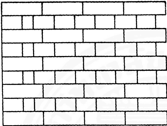
ENGLISH BOND
