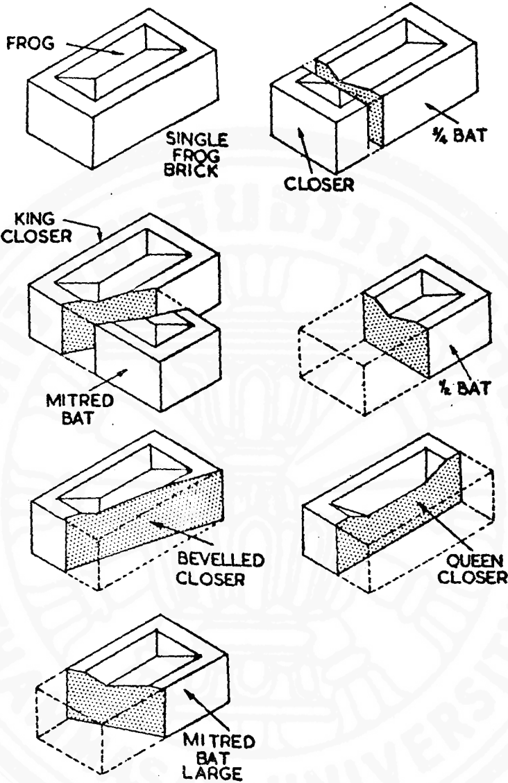
BRICK SHAPES IN COMMON USE. The standard shape brick is shown top left. The other shapes are cut from the standard brick.
