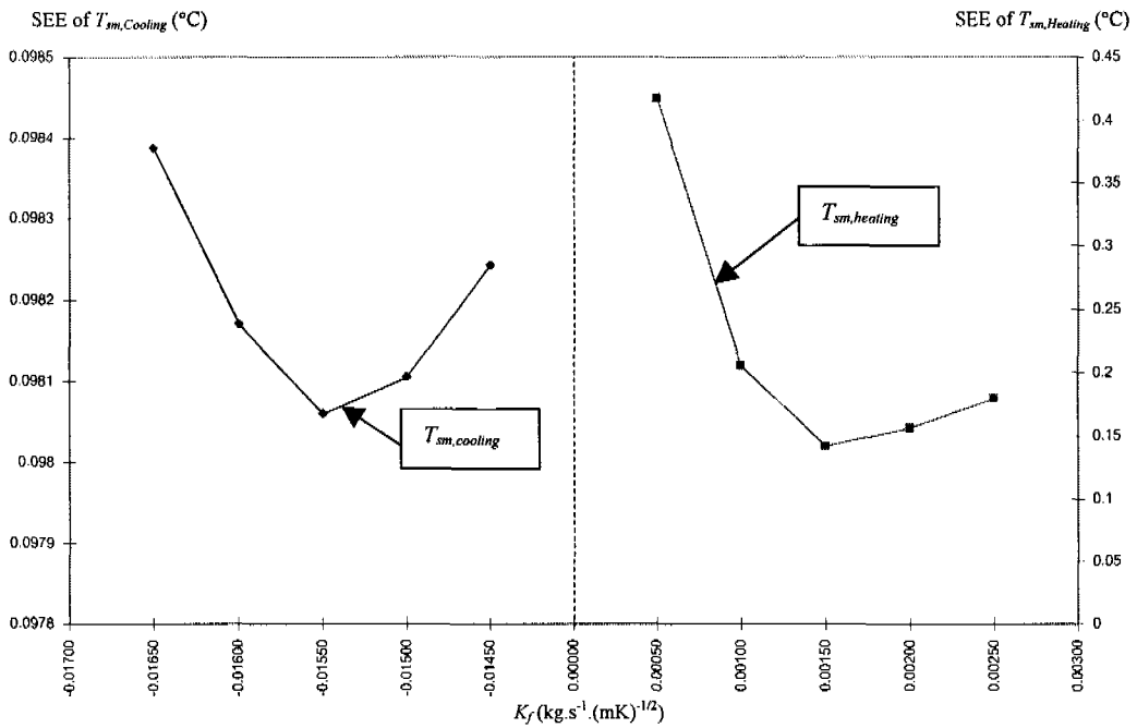
Fig. B2 Standard errors of estimate of T_{sm} found at different values of K_f for Case 1 on 9/10/2002
