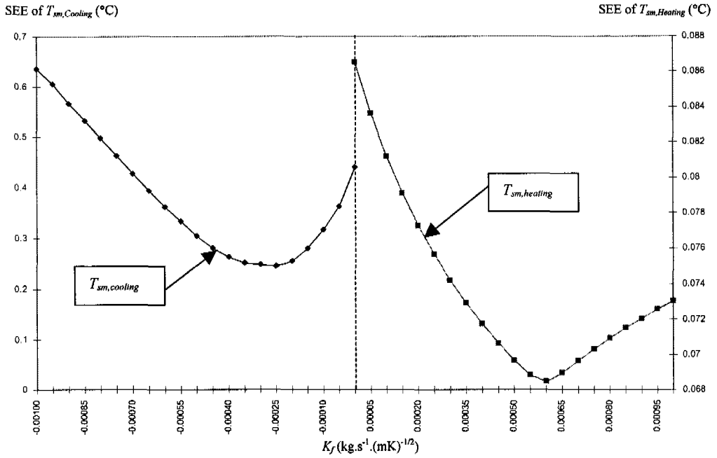
Fig. B1 Standard errors of estimate of T_{sm} found at different values of K_f for Case 3 on 12/7/2002
