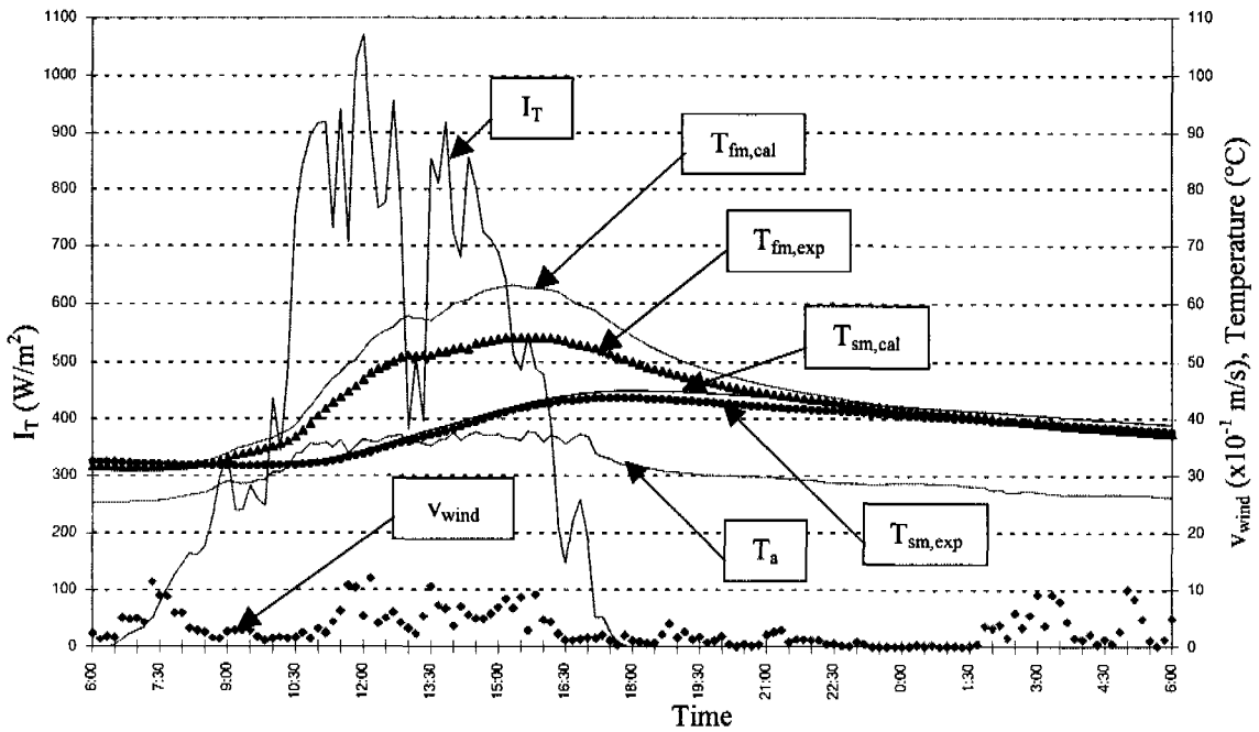
Fig. C4 Simulation results in comparison with experimental results on 13/11/2002
