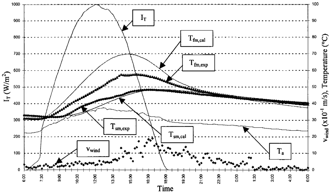
Fig. C3 Simulation results in comparison with experimental results on 11/10/2002
