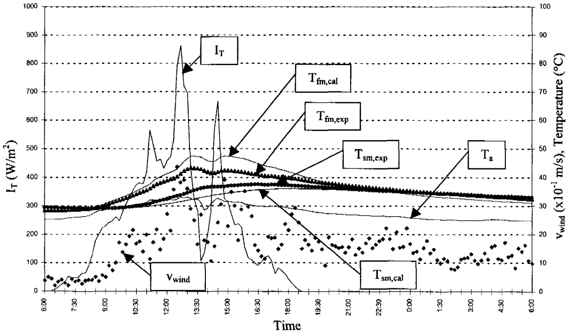
Fig. C1 Simulation results in comparison with experimental results on 17/8/2002
