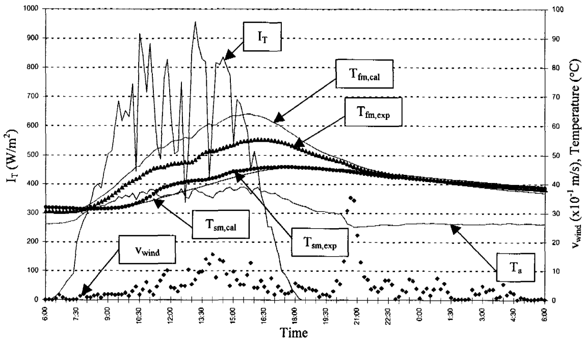
Fig. C2 Simulation results in comparison with experimental results on 3/10/2002
