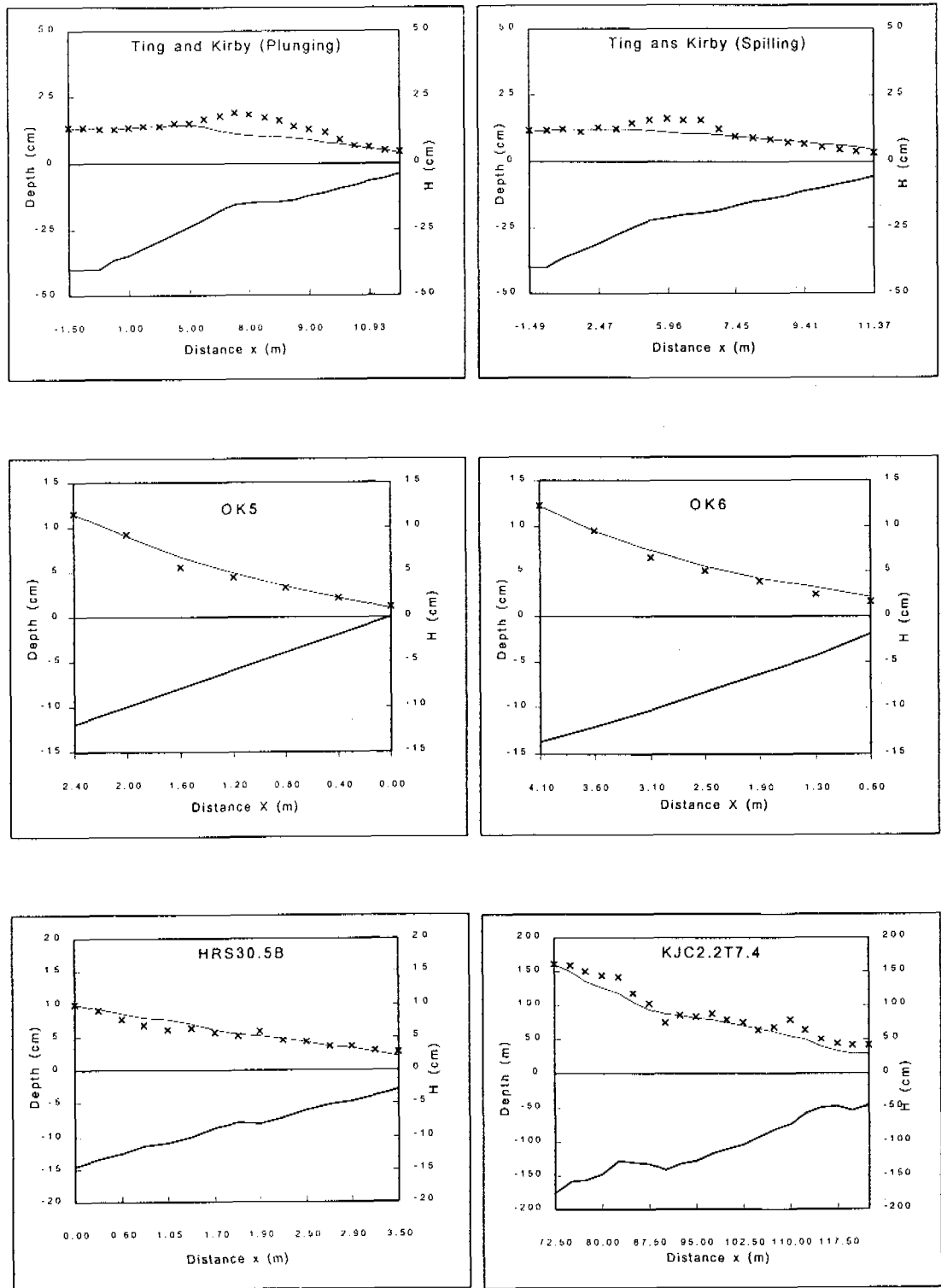
Fig. A.6 Computed wave height transformation compared with laboratory data of Ting and Kirby (1994), Okayasu (1988), Horikawa and Kuo (1966) and Kajima et al. (1983)
