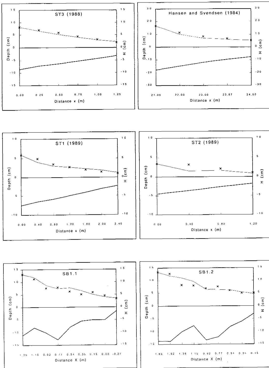
Fig. A.4 Computed wave height transformation compared with laboratory data of Sato (1988-1989), Hansen and Svendsen (1984) and Shibayama and Horikawa (1986)
