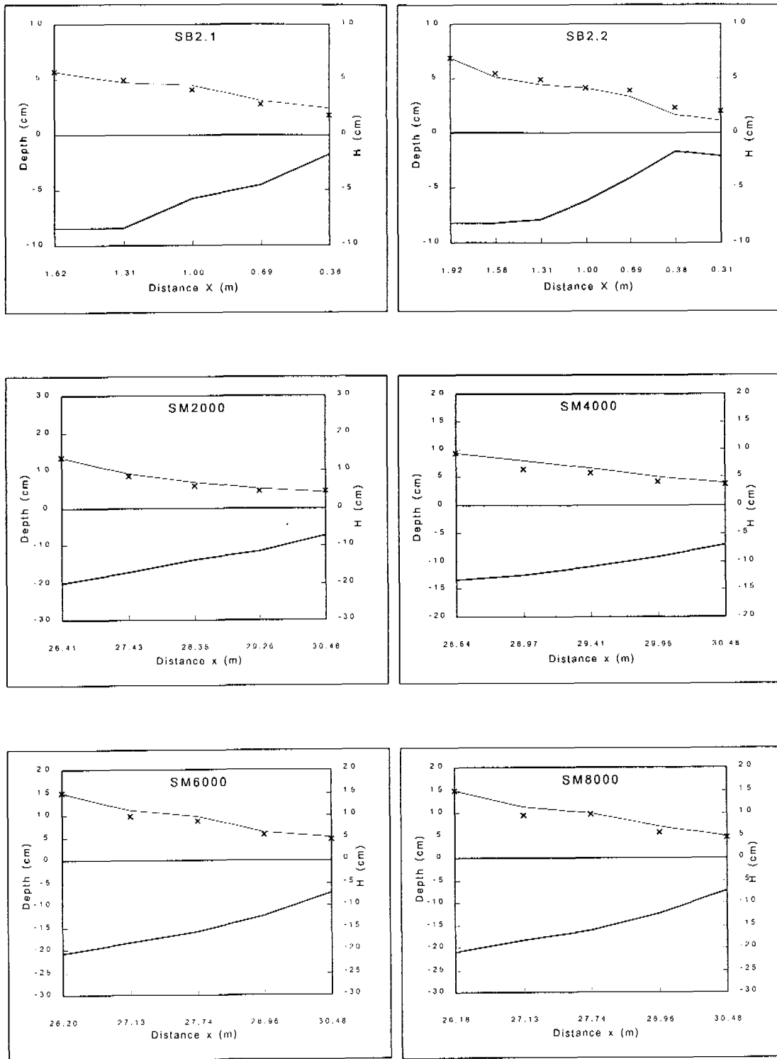
Fig. A.5 Computed wave height transformation compared with laboratory data of Shibayama and Horikawa (1986) and Smith and Kraus (1990)
