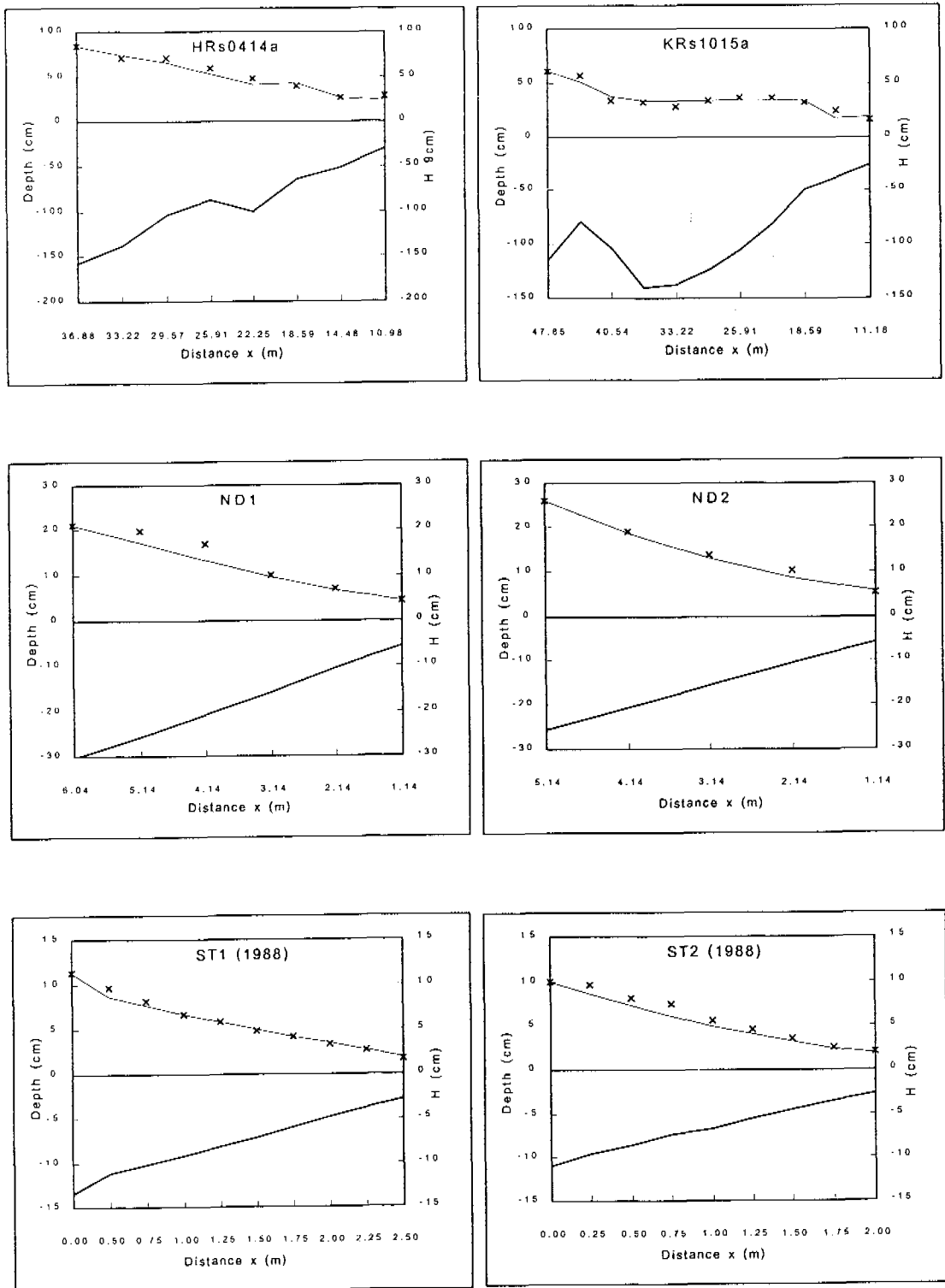
Fig. A.3 Computed wave height transformation compared with laboratory data of Kraus and Smith (1994), Nadaoka et al. (1982) and Sato (1988)
