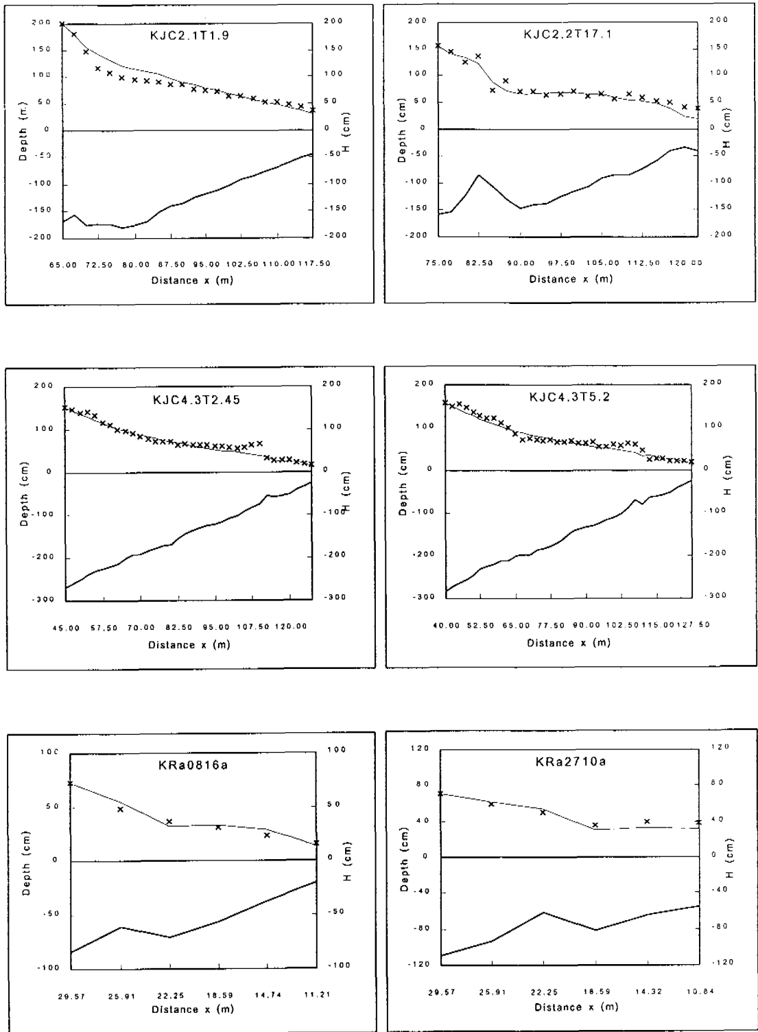
Fig. A.2 Computed wave height transformation compared with laboratory data of Kajima et al. (1983) and Kraus and Smith (1994)
