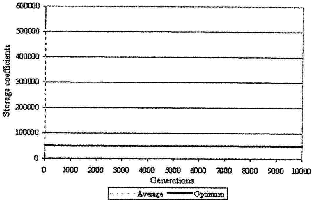
Fig. A.3 Relationship between optimum and average of storages and generations of mesh C3
